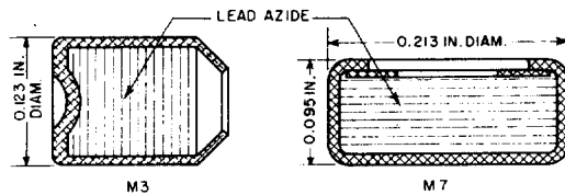
Fig 1 Typical Explosive Relays
